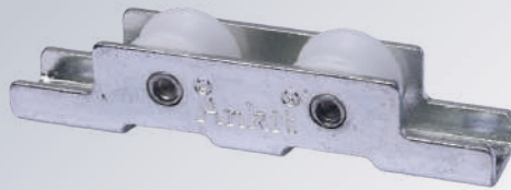
CODE: 9039 WHEEL: MLDG BRACKET: MS
